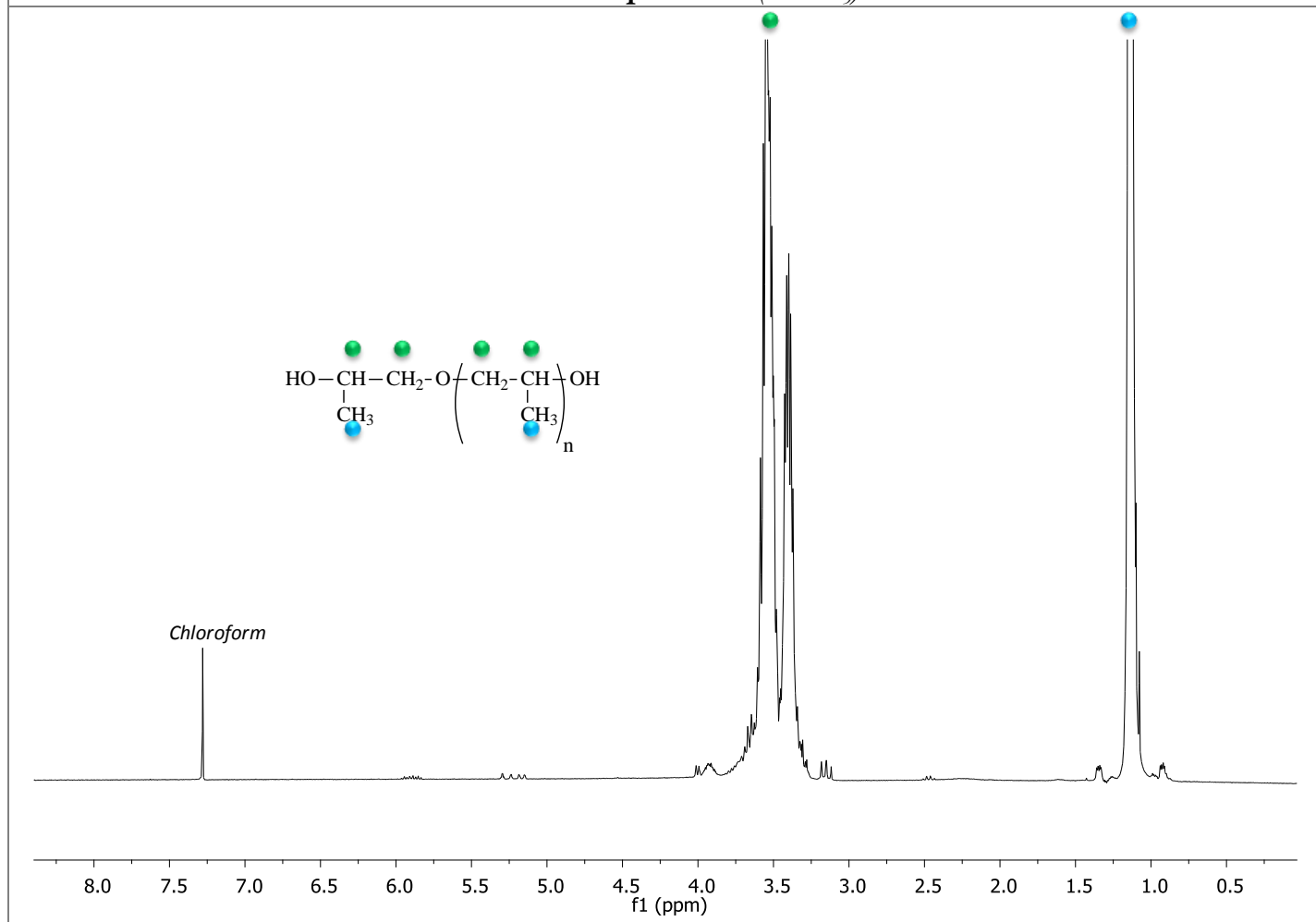
^1\text{H} NMR Spectrum ( \text{CDCl}_3 )
