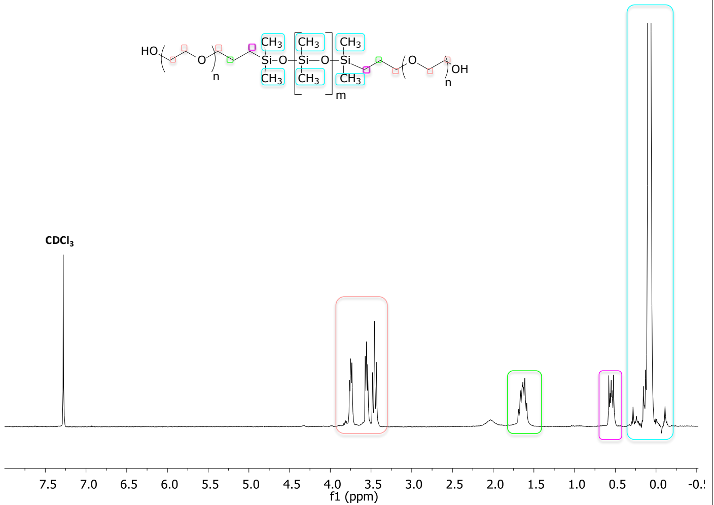
1 H NMR Spectrum ( Deterated Chloroform )
