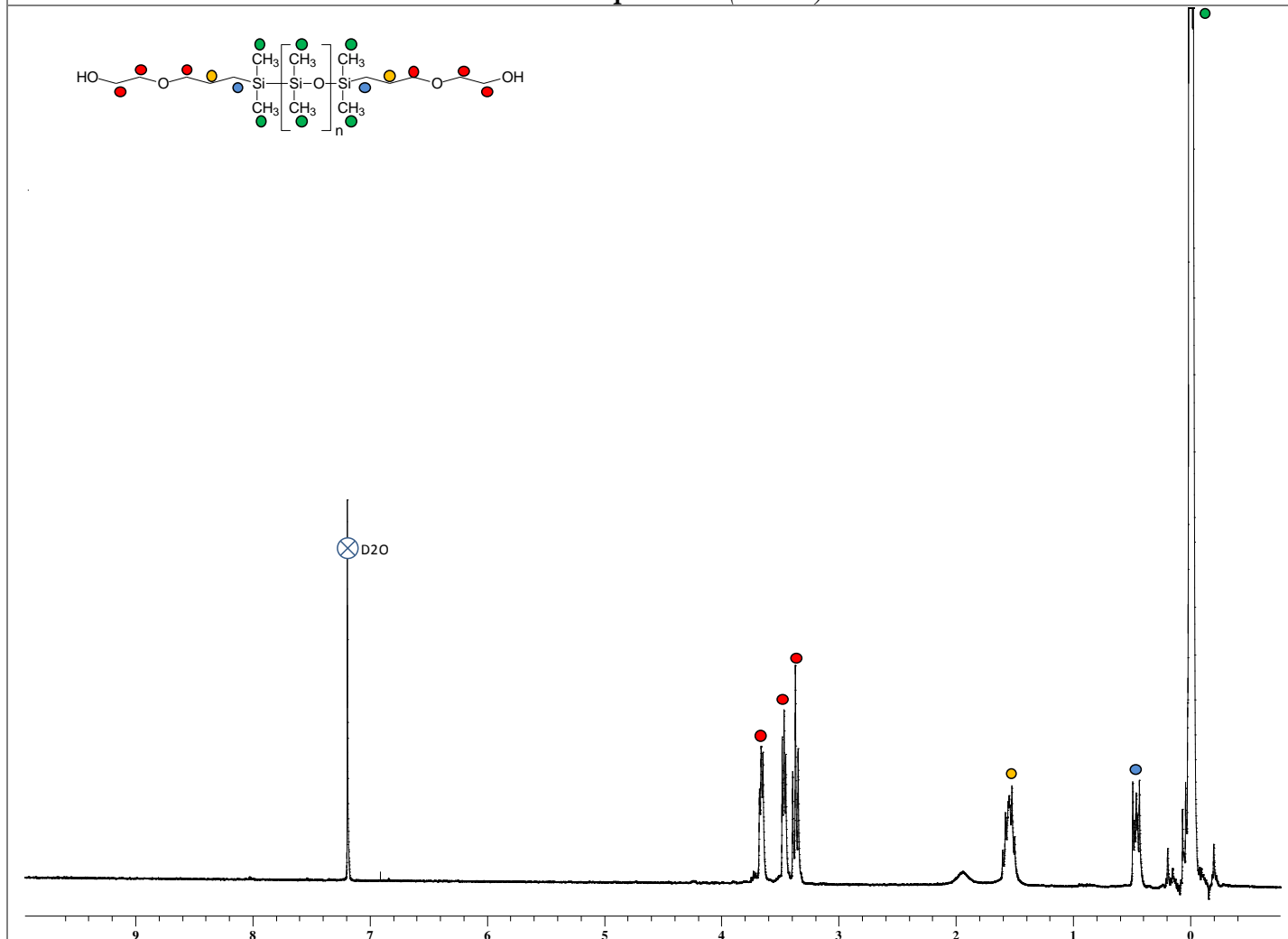
^1\text{H} NMR Spectrum ( \text{CDCl}_3 )
